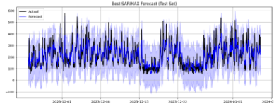
Fig. 10. SARIMAX forecast on the test set.
