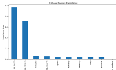
Fig. 13. XGBoost feature importance scores.
