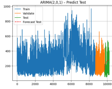
Fig. 8. ARIMA model prediction on test set.
